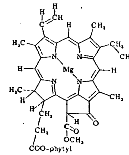
Chlorophyll a
